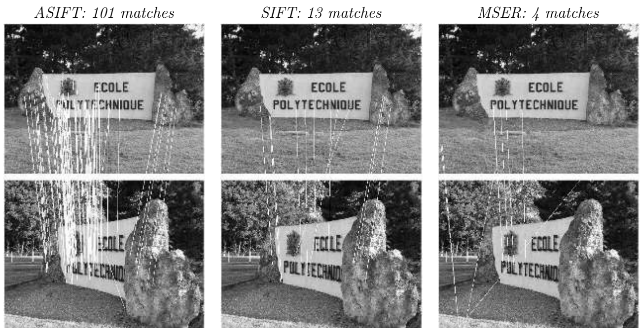
Figure 21: École Polytechnique, pictures at frontal view and at 65 degree angle, absolute tilt t = 2.4 . Not shown: Harris-Affine (2 matches), Hessian-Affine (2 matches).
